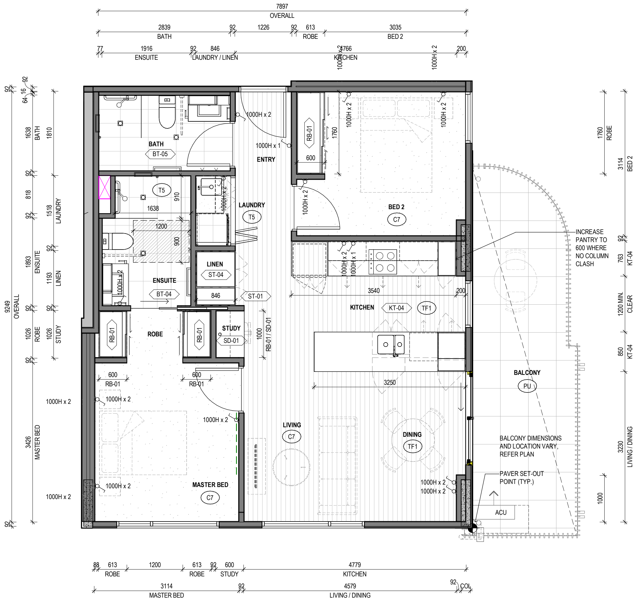
1 ILA Type 6 Scale 1: 50
